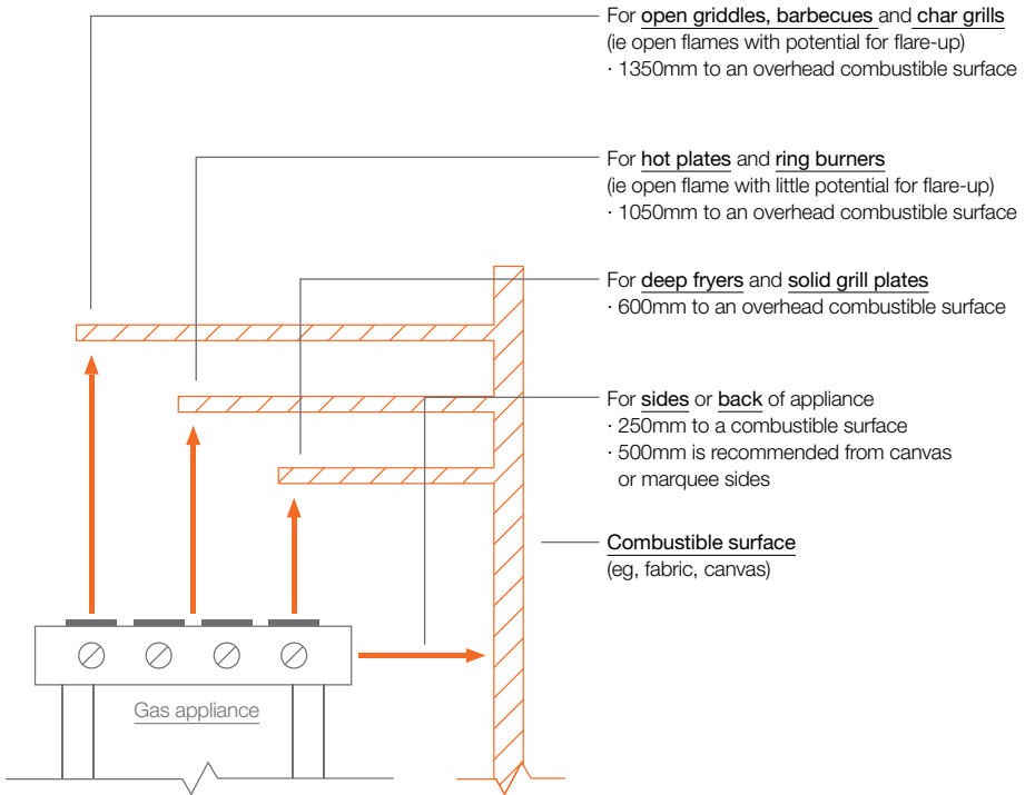
Figure 3: Appliance clearances from combustible material
