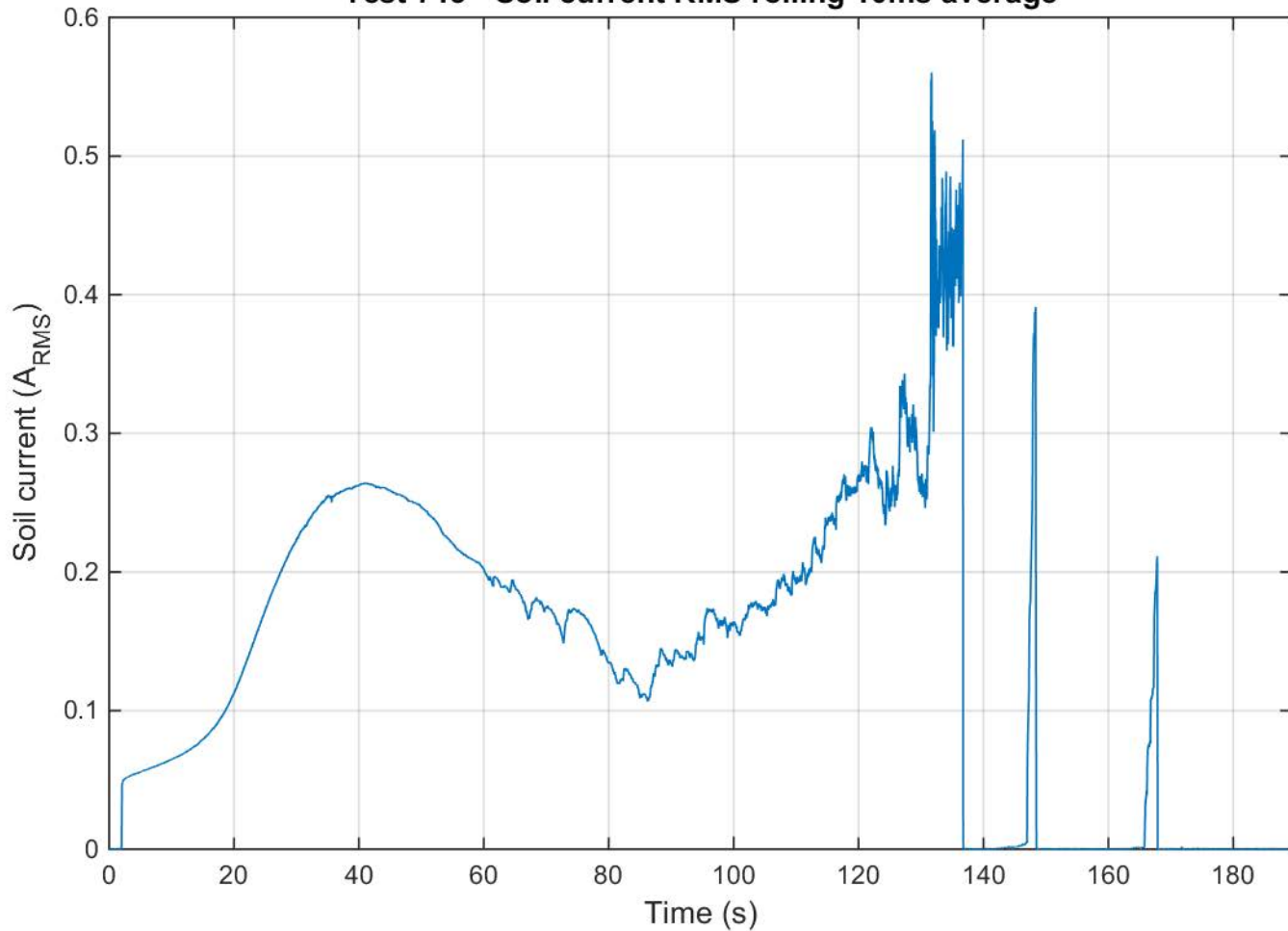
Test 715 - Soil current RMS rolling 10ms average
