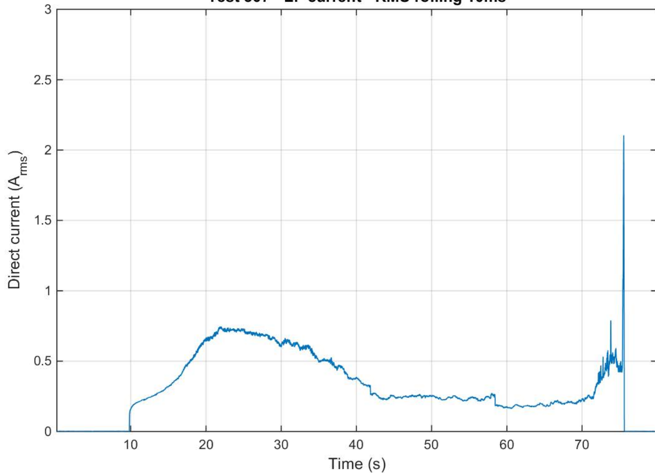
Test 307 - LF current - RMS rolling 10ms
